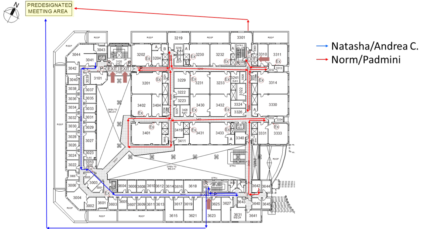
Figure 9 Key Plan of the Third Floor of the FSC. Standpipes (not marked) are located in stairwells 2, 3, and 4 (NW, NE, and SE stairwells).
