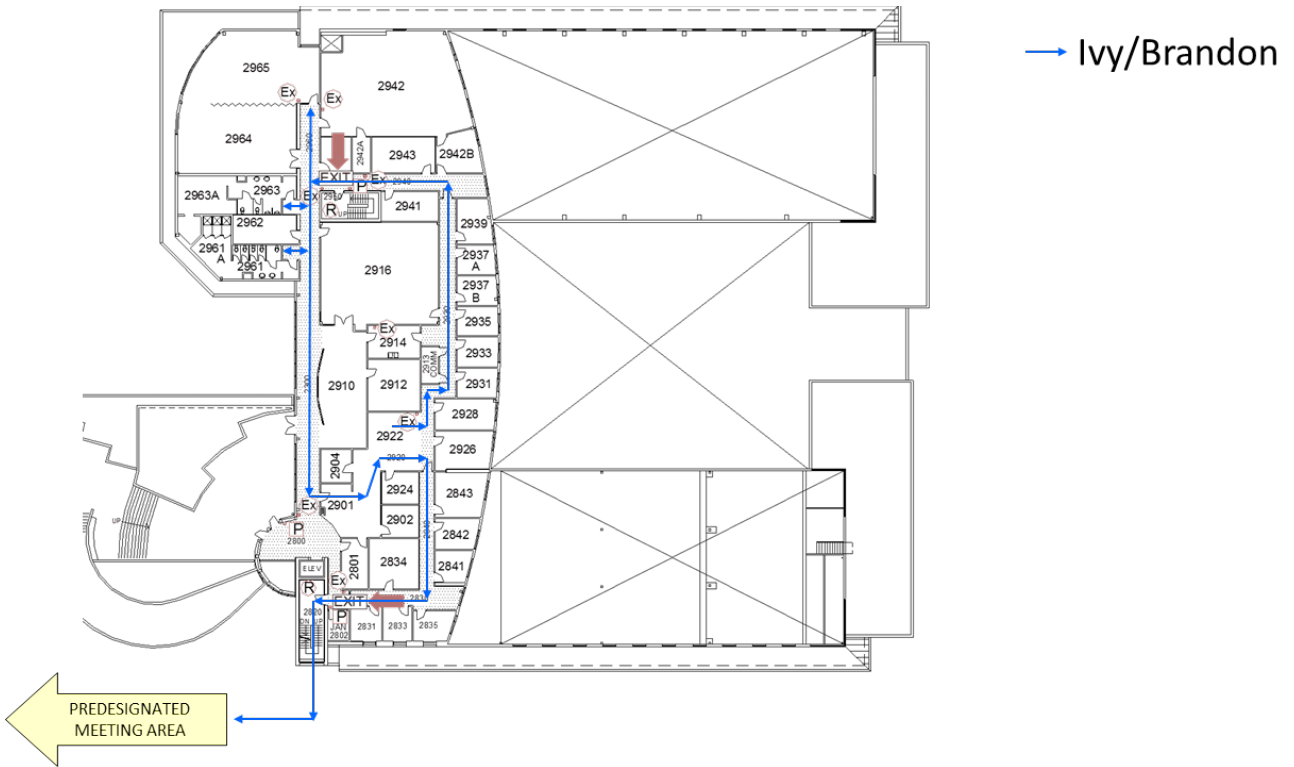
Figure 8 Key Plan of the Second Floor of CAWP (enlarged view).
