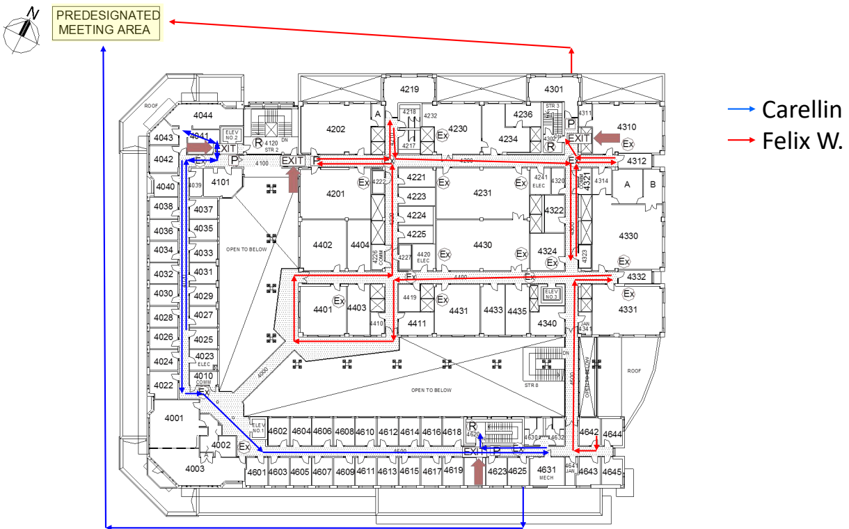
Figure 10 Key Plan of the Fourth Floor of the FSC. Standpipes (not marked) are located in stairwells 2, 3, and 4 (NW, NE, and SE stairwells).
